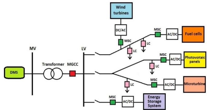
Fig. 11. An example of the hierarchical control layout of the architecture and structure of the MG with MGCC and MSC [13].
