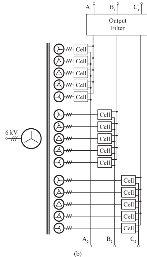
Fig. 4. CHB topology with isolated cell supply transformer with a) cell outputs connected in series for shunt current injection and b) cell outputs connected in parallel for series voltage injection.
