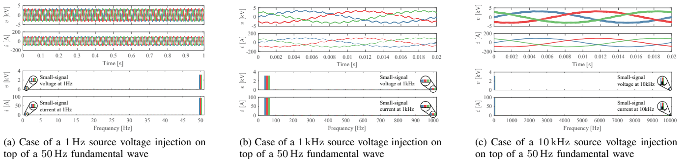
Fig. 11. Simulation waveforms for the configuration in Fig. 2a. a , b and c phase voltages and currents are visible in blue, red and green.
