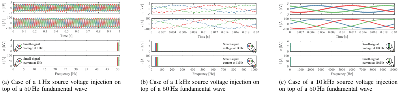
Fig. 12. Load side simulation waveforms for the configuration in Fig. 2b. a , b and c phase voltages and currents are visible in blue, red and green.
