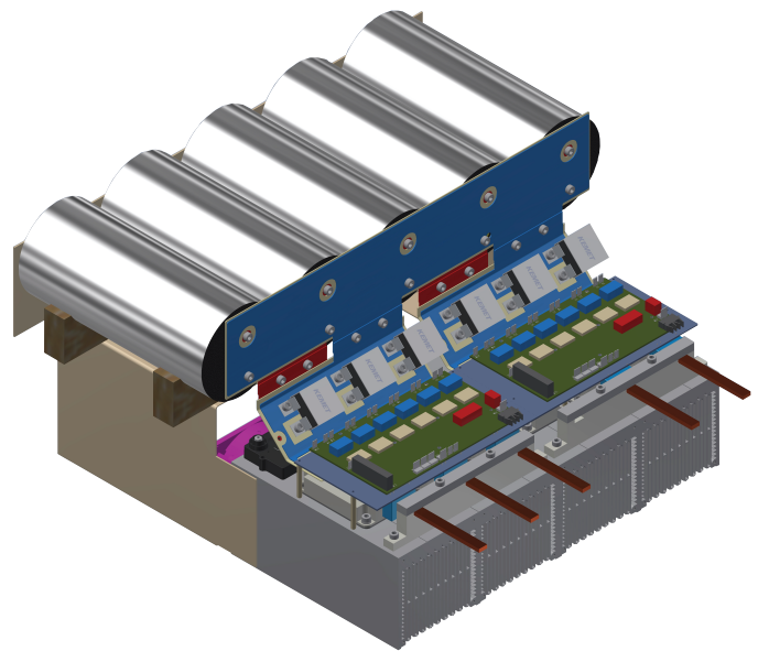
Fig. 9. 3D CAD representation of the cell. AFE is to positioned to the left side and HB inverter to the right.
