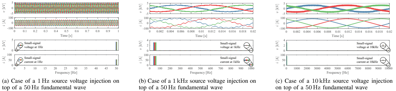
Fig. 13. Source side simulation waveforms for the configuration in Fig. 2c. a , b and c phase voltages and currents are visible in blue, red and green.
